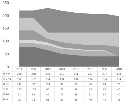
Advance of the Gas / Water contact per block since 2011 1/3 (meters)
