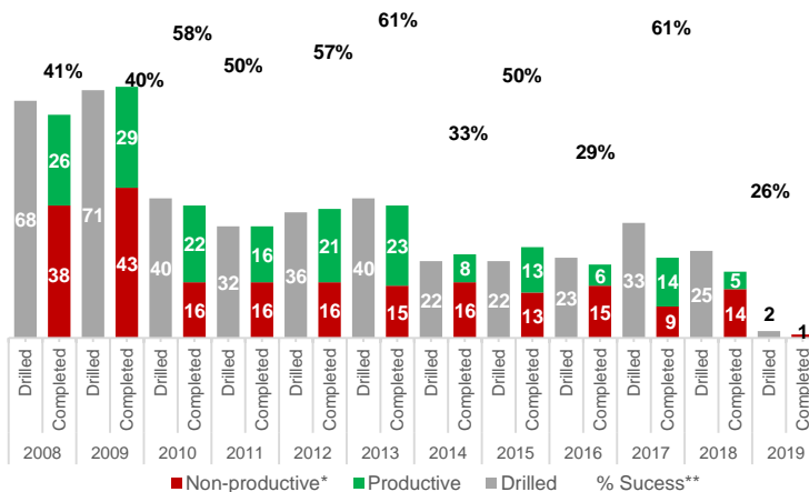
Historic drilling and well completion 2008-2019
