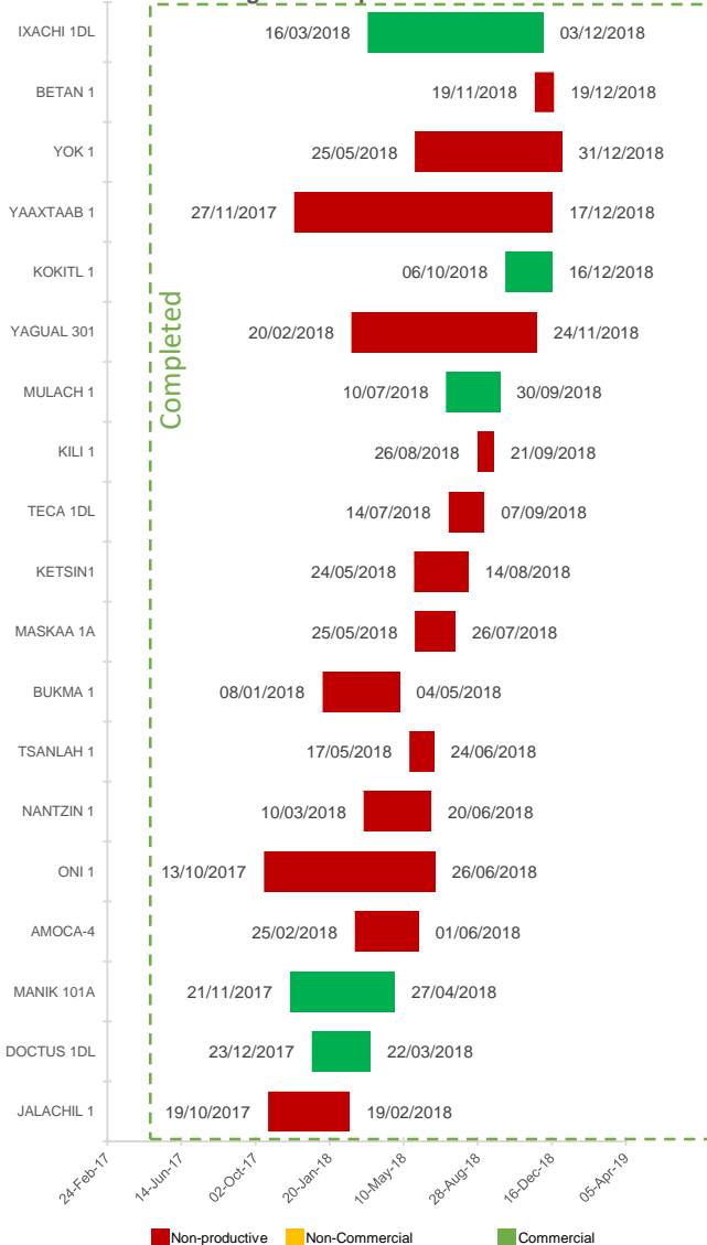
Drilling and completion dates
